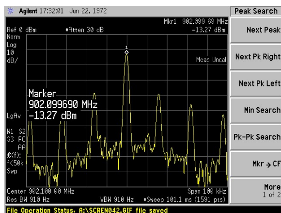
Figure 6 Marker at 902 MHz
